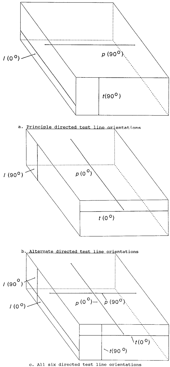
FIG. 7 Schematic Showing the Six Possible Directed Test Line Orientations for Grain Size Measurement
